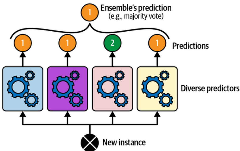
Figure 7-2. Hard voting classifier predictions
